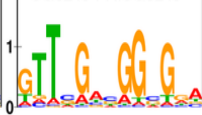
CG5245-PA:CG5245
