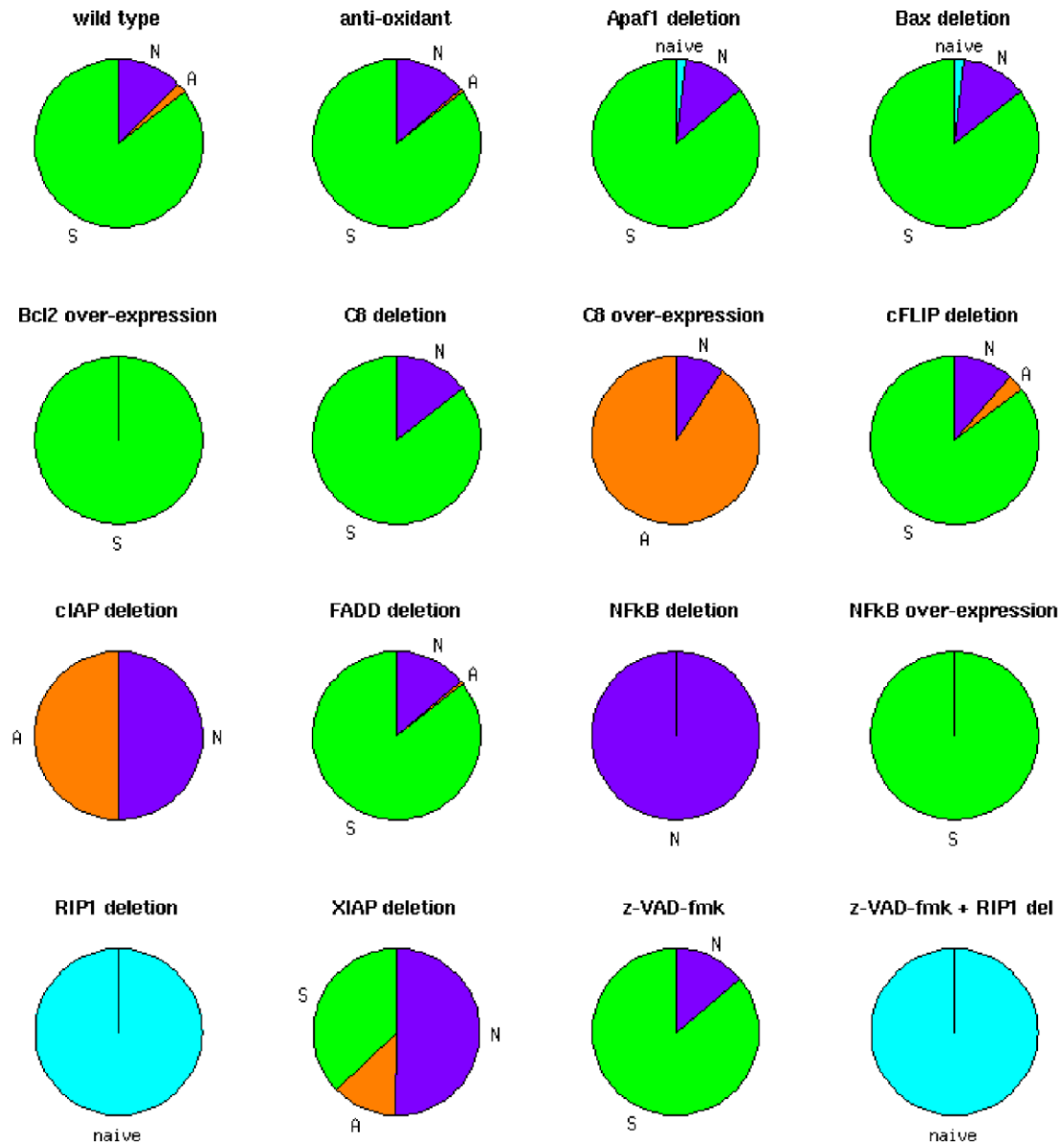
Supp. Figure S1. Simulations of the reduced cell fate model incremented by the interaction cIAP \dashv CASP8 with TNF=1 , FasL=0 .
