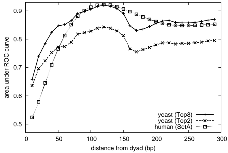
Figure S9: Area under the ROC curve as a function of the distance L between the dyad positions and the non -dyad positions on either side. Near the dyad, discrimination is difficult and the performance is not much better than random, especially in human. As the distance from the dyad increases, performance improves, reaching a maximum in the linker, after which the performance degrades again.
