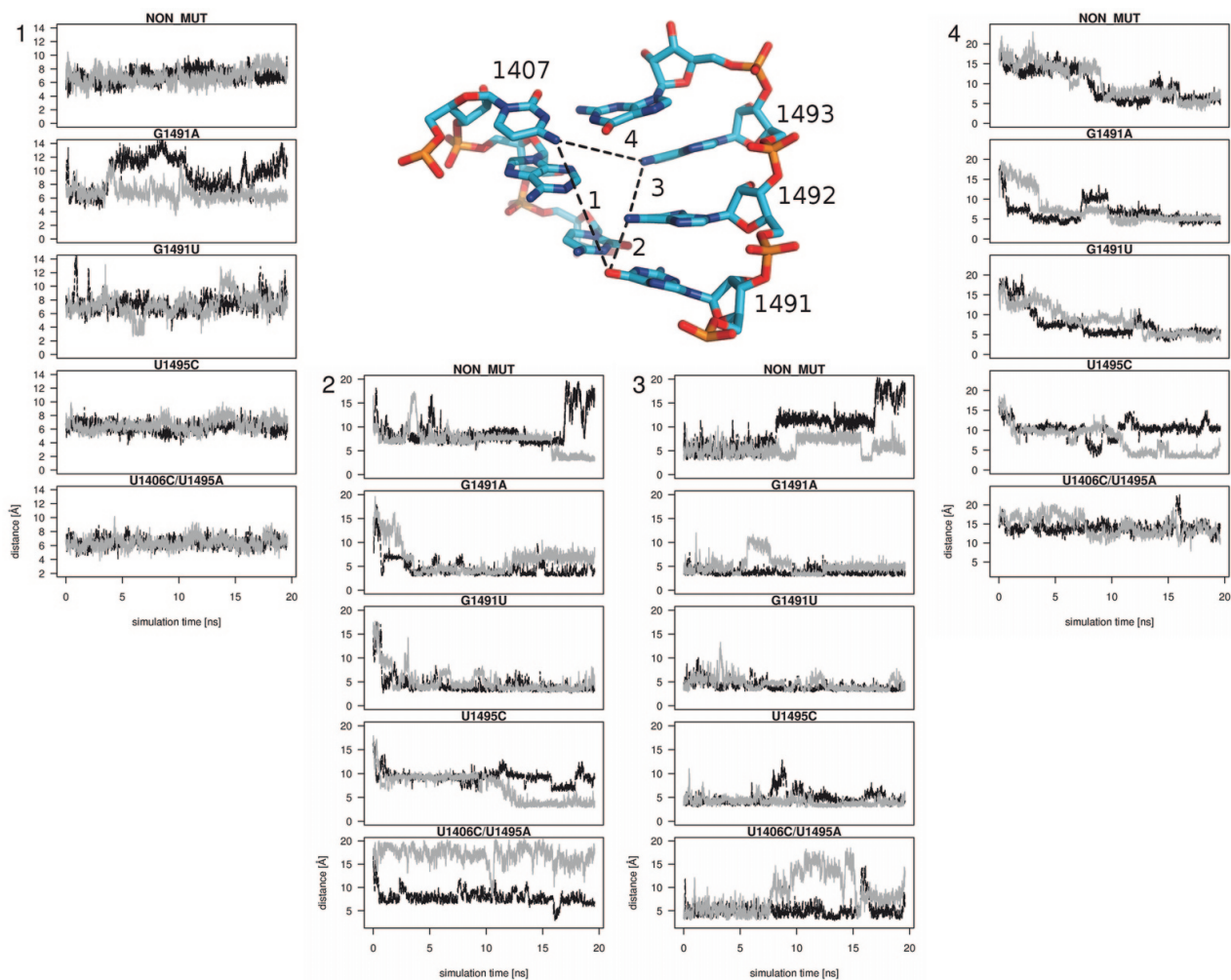
Figure S5: Distances between chosen atoms inside the A-site as a function of the simulation time. Four sets of graphs correspond to four distances (1, 2, 3, 4) depicted as black dotted lines on a stick model of the A-site fragment; for base numbering see Figure 1a. Grey and black lines are for two simulated A-sites.
