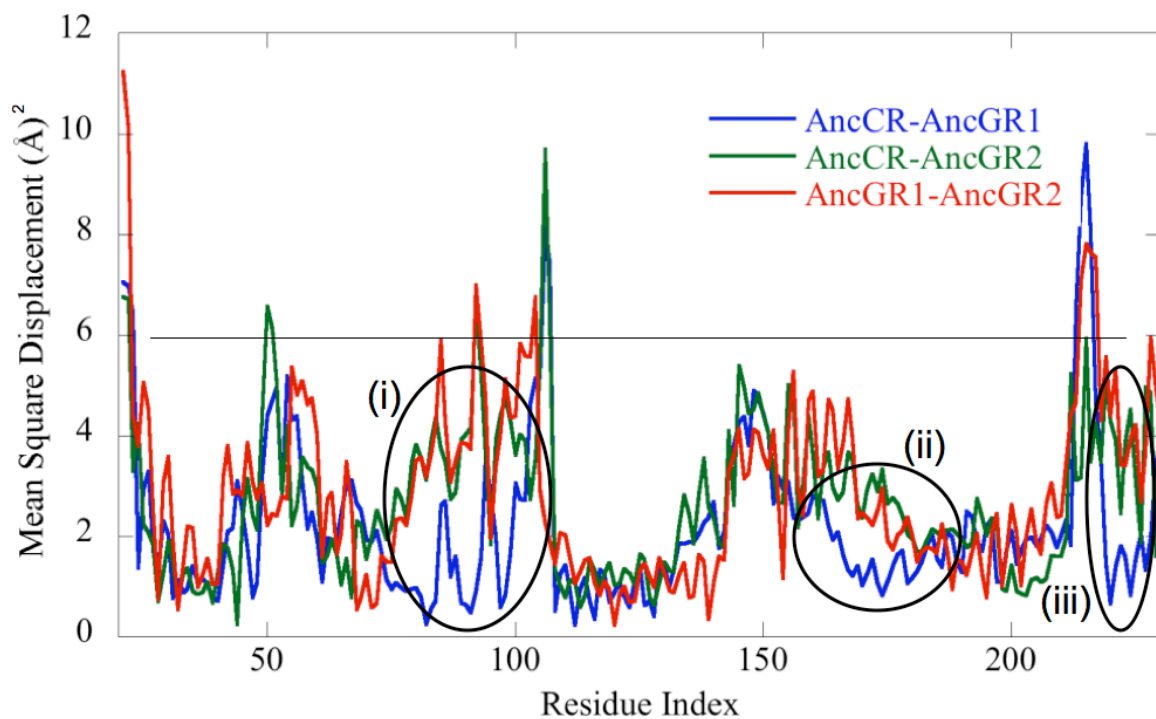
Fig. S2: The Mean Square Displacement between our predicted structures for AncCR-AncGR1 (blue), AncCR-AncGR2 (green), and AncGR1-AncGR2 (red). The three large structural changes between successive generations are associated with the shift in; (i) \beta -sheet b1 and helices 5, 6 and 7; (ii) helix 9 and the top of helix 10; (iii) the bottom loop of helix 10 and the activation function helix.
