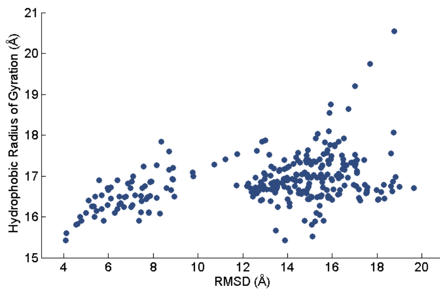
Fig. S6: Radius of gyration of the hydrophobic residues versus the rmsd from the experimentally determined structure of AncCR for a single FRODA run. By using the hydrophobic radius of gyration we select against non-native like structures and only seed the ensuing REMD simulations with collapsed structures, many of which are native-like.
