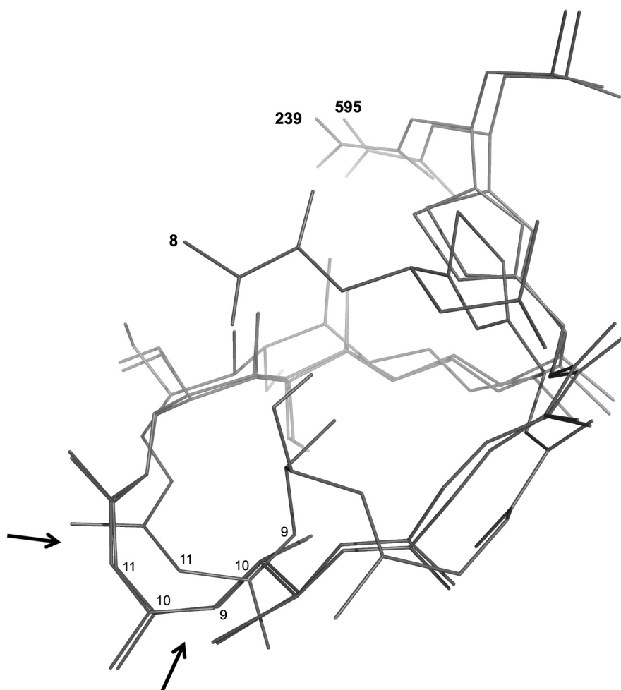
Figure S2: Computed low energy conformations d8 , d239 , d595 of Archazolid A. The conformers display torsion angles close to 55^\circ between the double bonds in positions 9 and 11 (arrows).
